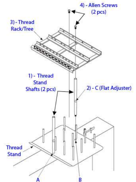
Image 1 – Thread Rack
